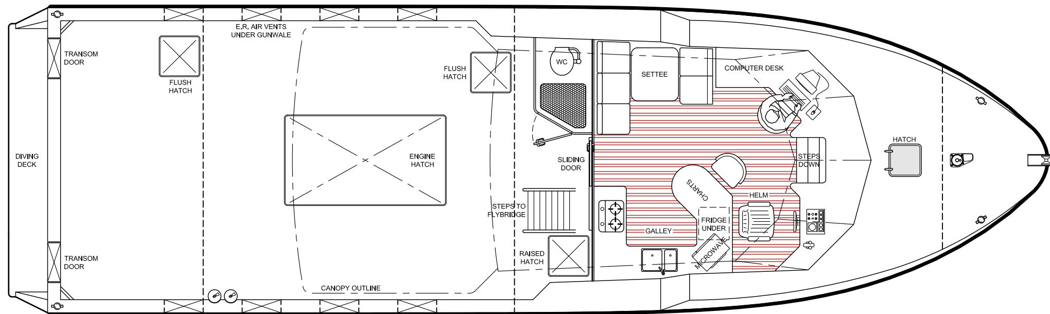
PLAN ON MAIN DECK
