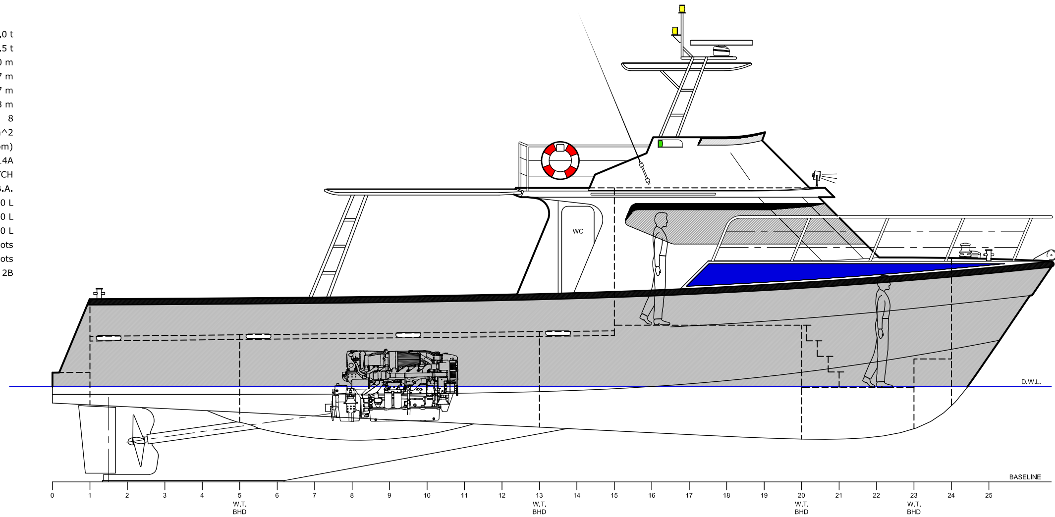
OUTBOARD PROFILE
