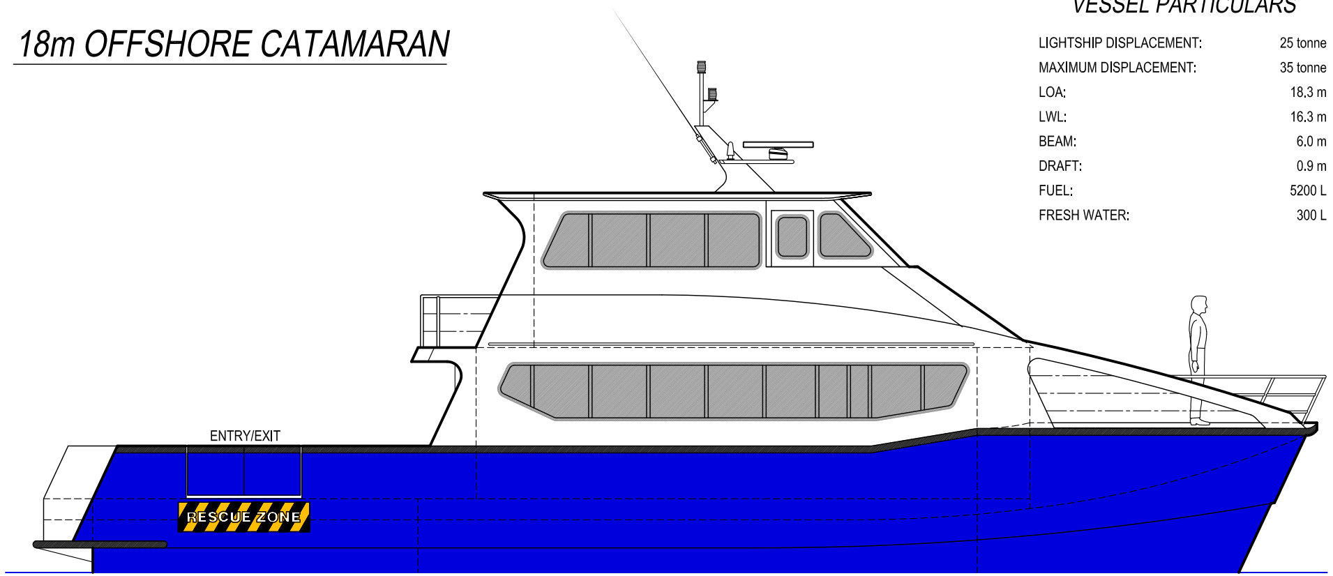
STBD PROFILE
