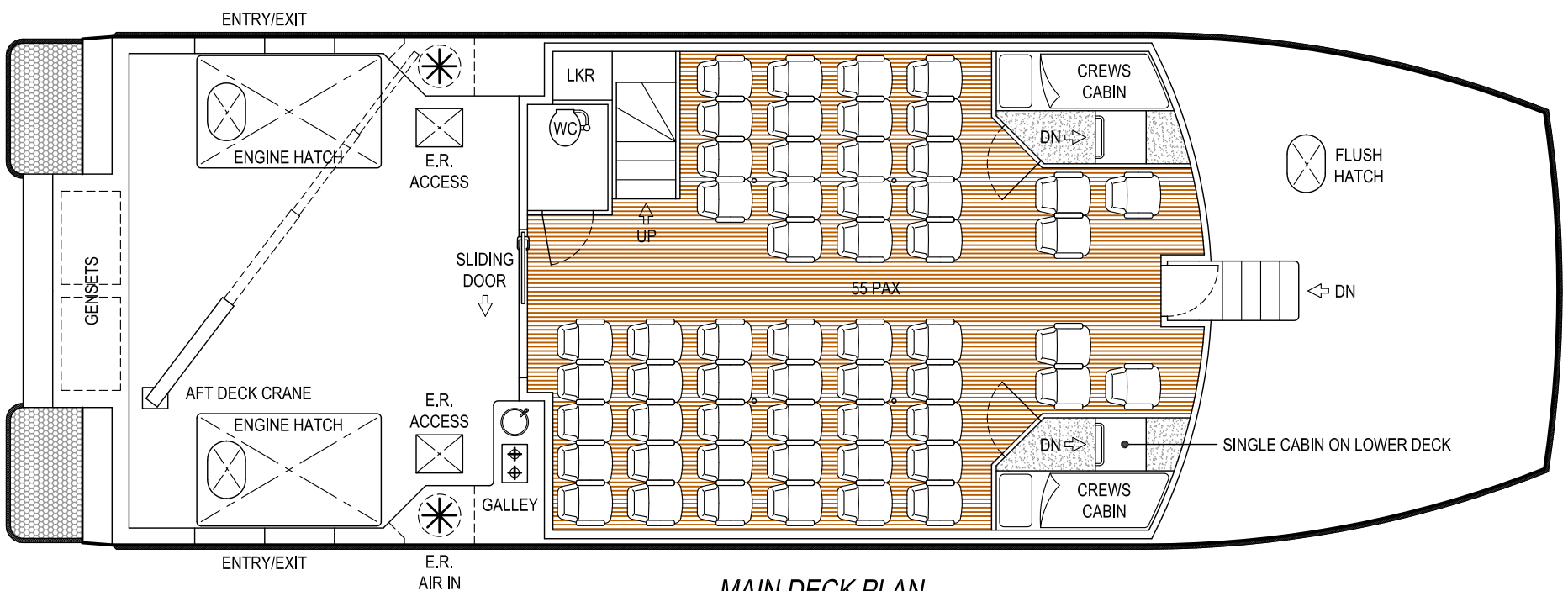
MAIN DECK PLAN
