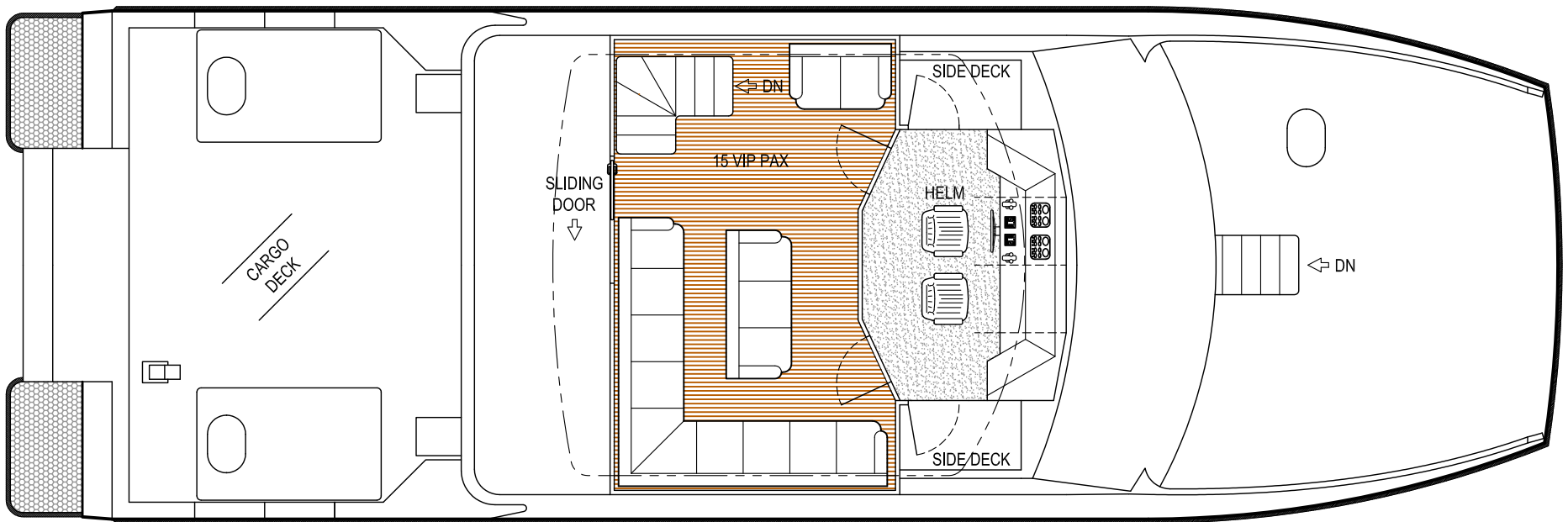
UPPER DECK PLAN
