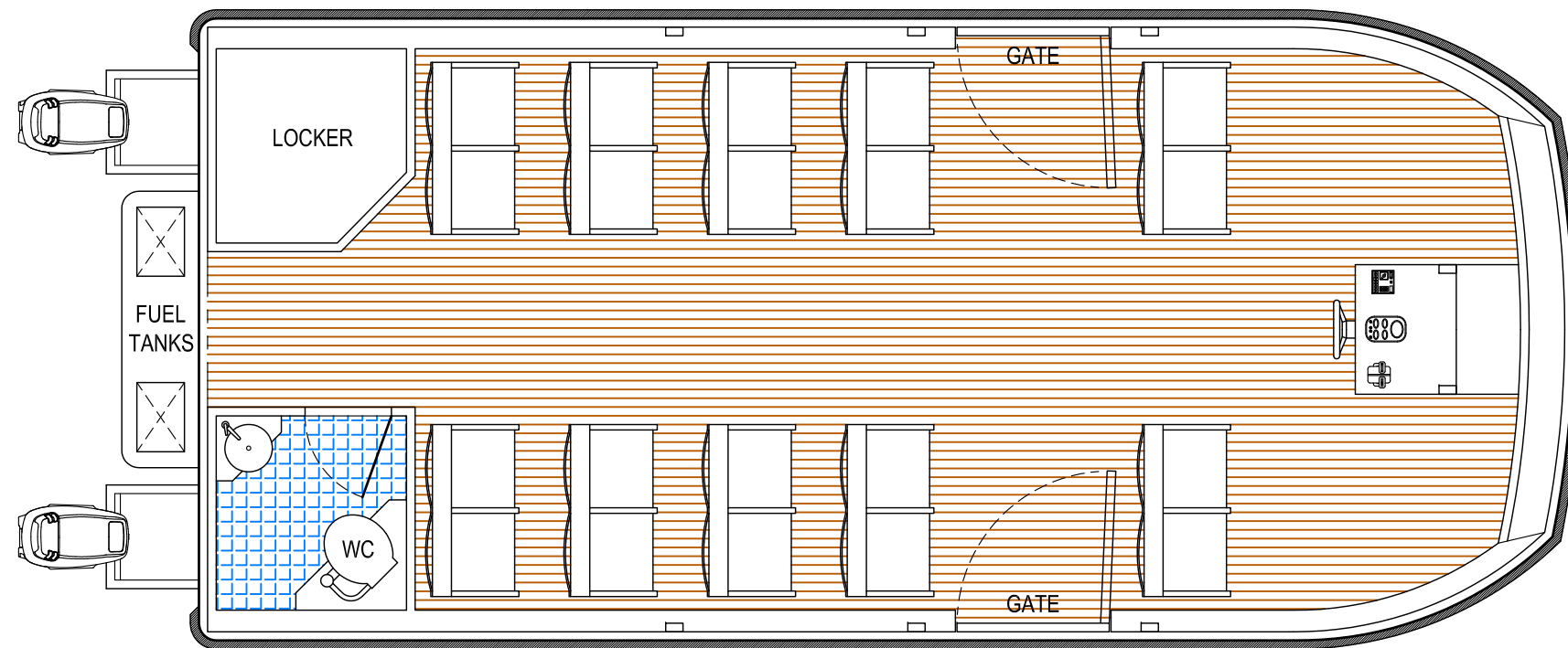
DECK PLAN
